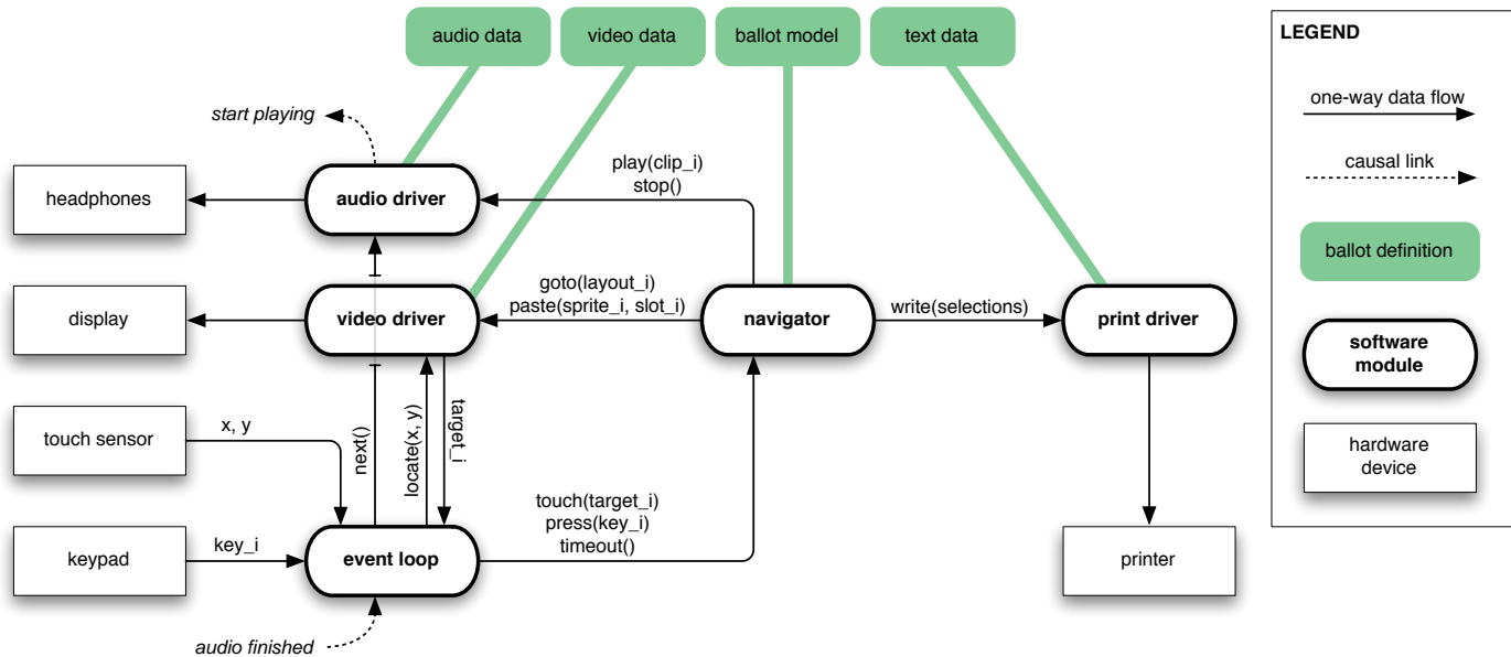
Figure 6.1: Block diagram of the virtual machine, which consists of the five software modules in bold. The arguments clip_i , layout_i , sprite_i , target_i , key_i , x , and y are integers; selections is a list of lists of integers.
